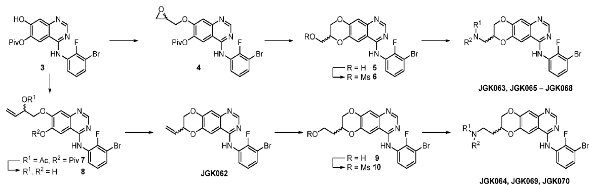
Scheme 2. Synthesis of JGK063 – JGK070.
