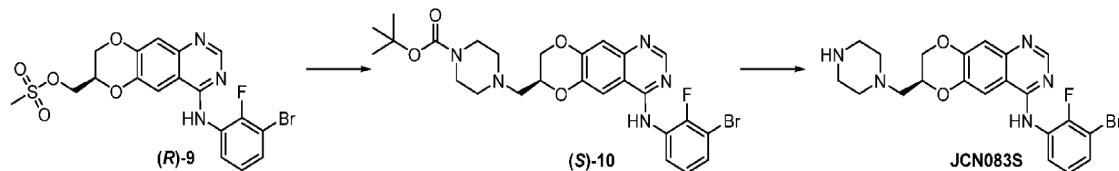
Scheme 4. Synthesis of JGK083S.
