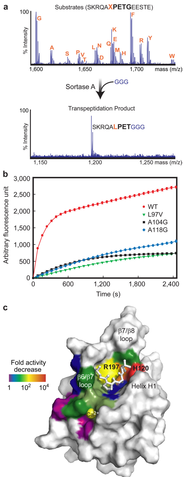
FIGURE 5. The structure of the SrtA _{\Delta N59} -LPAT* complex is compatible with biochemical data. a , data showing that SrtA only recognizes sorting signals that contain a leucine residue at the first position of the LPXTG motif. Shown are MALDI-TOF spectra of a peptide library containing a sorting signal randomized at the leucine position before ( top ) and after ( bottom ) incubation with SrtA and its second substrate Gly 3 . Each peptide contains the sequence SKRQAXPETGEESTE, where X is any amino acid except for Ile or Cys. The results of this assay show that SrtA specifically recognizes leucine within the
