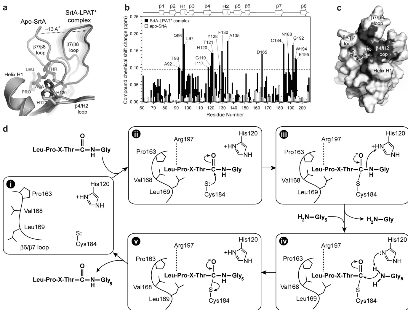
FIGURE 8. Localization of the lipid II binding site and proposed mechanism of transpeptidation. a , superposition of the NMR structures of apo-SrtA ΔN59 (34) (Protein Data Bank code 1ija) and the SrtA ΔN59 -LPAT* complex. The image shows an expanded view of the substrate-dependent structural change in the β7/β8 loop that unmask a groove leading into the active site. The image was generated in a similar manner as the one shown in Fig. 3 b . b , histogram plot of the compound chemical shift changes for the backbone amide hydrogen and nitrogen atoms of SrtA ΔN59 after the addition of the Gly 3 tripeptide. Chemical shift changes after the addition of the peptide to either the SrtA ΔN59 -LPAT* complex (black) or SrtA ΔN59 in its apo-state (white) are shown. The secondary structure of the enzyme and amino acids experiencing the largest changes are labeled. The data indicate that only SrtA in the context of the SrtA ΔN59 -LPAT* complex binds to the Gly 3 tripeptide. The dashed line represents one S.D. above the average chemical shift perturbation of all amino acids. c , solvent-accessible surface of SrtA ΔN59 in the complex with residues that are significantly perturbed by the addition of the Gly 3 peptide colored dark gray. The majority of the chemical shift changes occur near the active site around the surface uncovered when the β7/β8 is displaced from helix H1. d , transpeptidation mechanism based on the structure of the SrtA ΔN59 -LPAT* complex and biochemical data. i , apoenzyme containing a flexible β6/β7 loop; ii , sorting signal binding closes the β6/β7 loop. Arg 197 hydrogen-bonds to the backbone, and the threonine carbonyl carbon is attacked by the thiolate of Cys 184 . iii , the displaced β7/β8 loop serves as an exit point for residues COOH-terminal to the LPXTG motif. This enables His 120 to protonate the amide of the glycine residue as the scissile bond is broken. iv , the cross-bridge peptide of lipid II enters the active site via the surface unmasked by the movement of the β7/β8 loop. v , a second tetrahedral intermediate forms, followed by the rupture of the Cys 184 -sorting signal linkage and product release.
