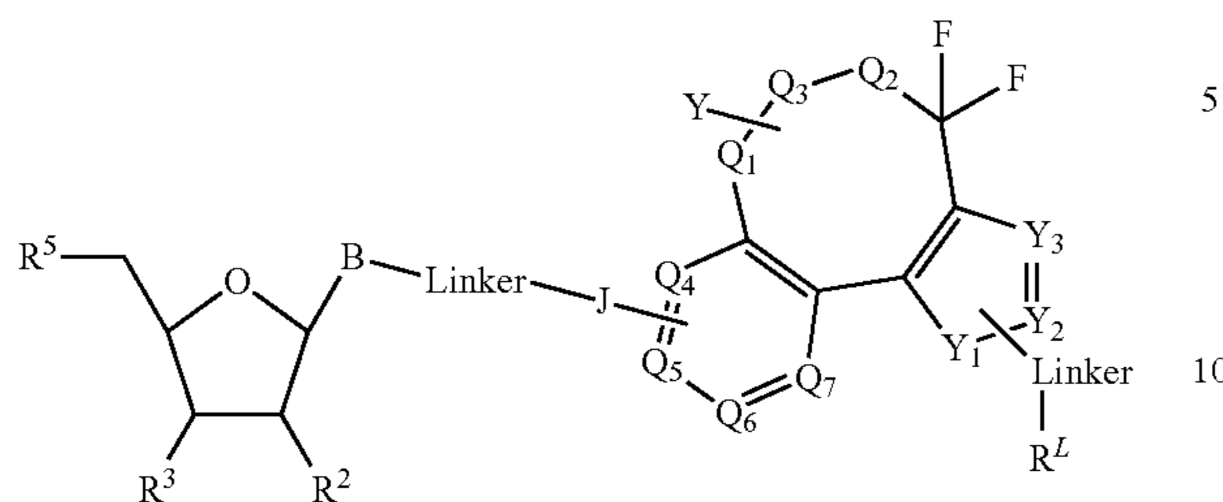
Formula (XVb)
