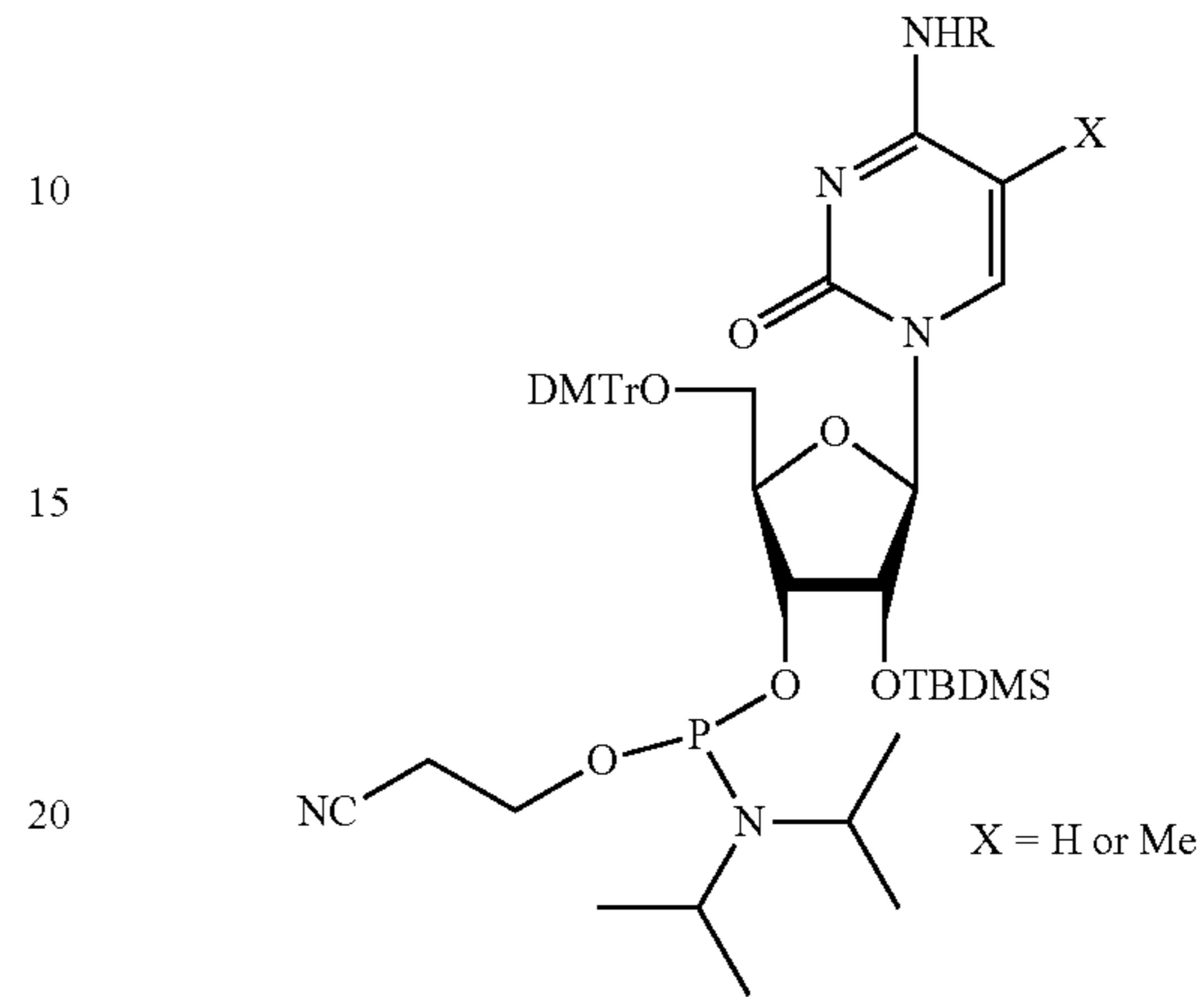
Scheme 17
