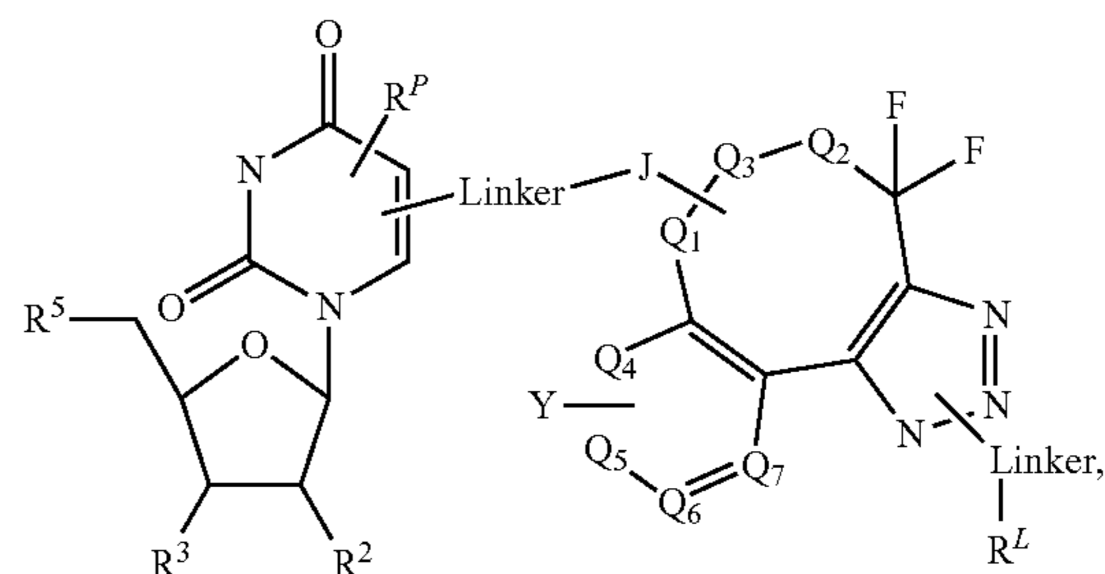
Formula (XVIIa)
