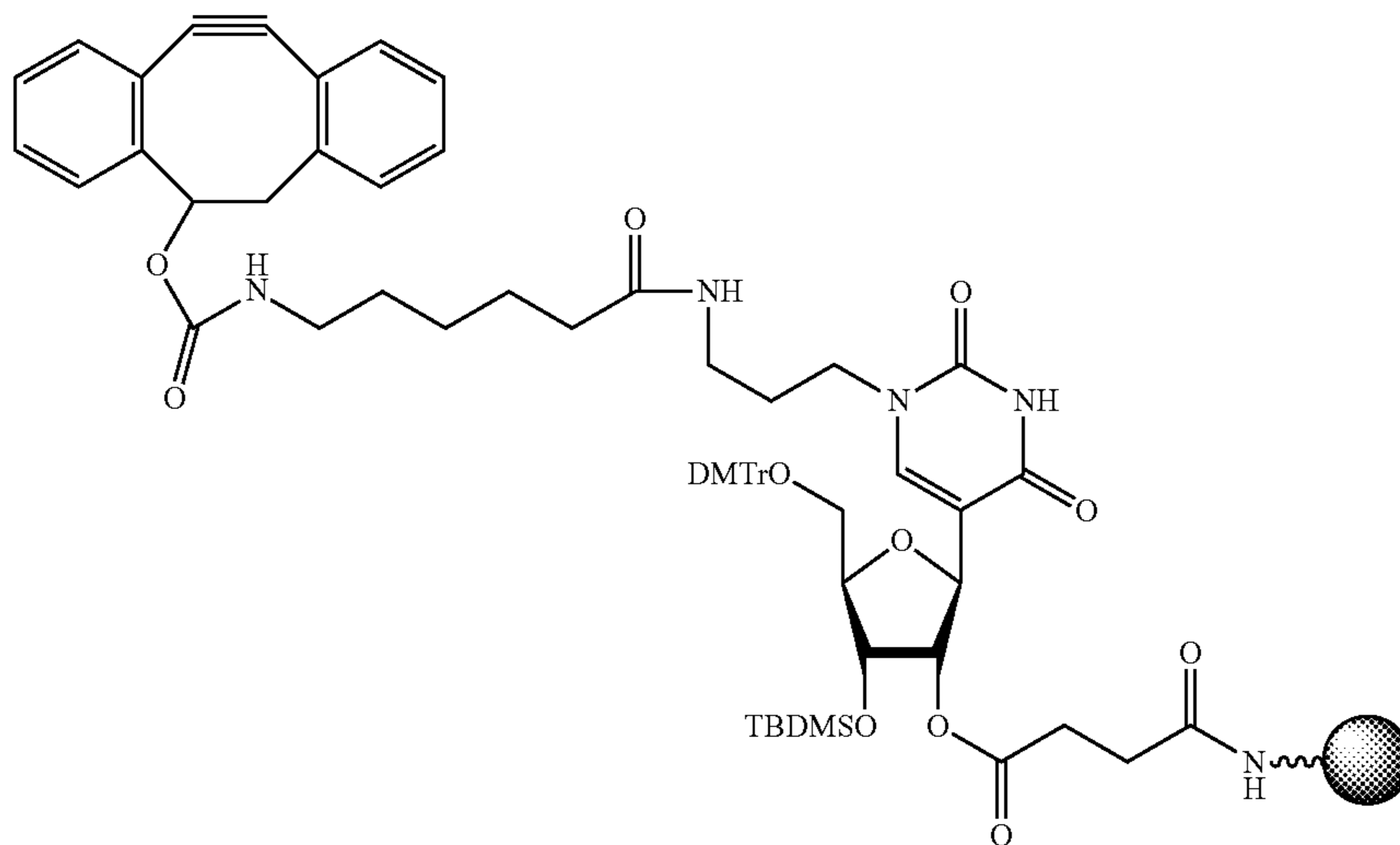
Scheme 20
