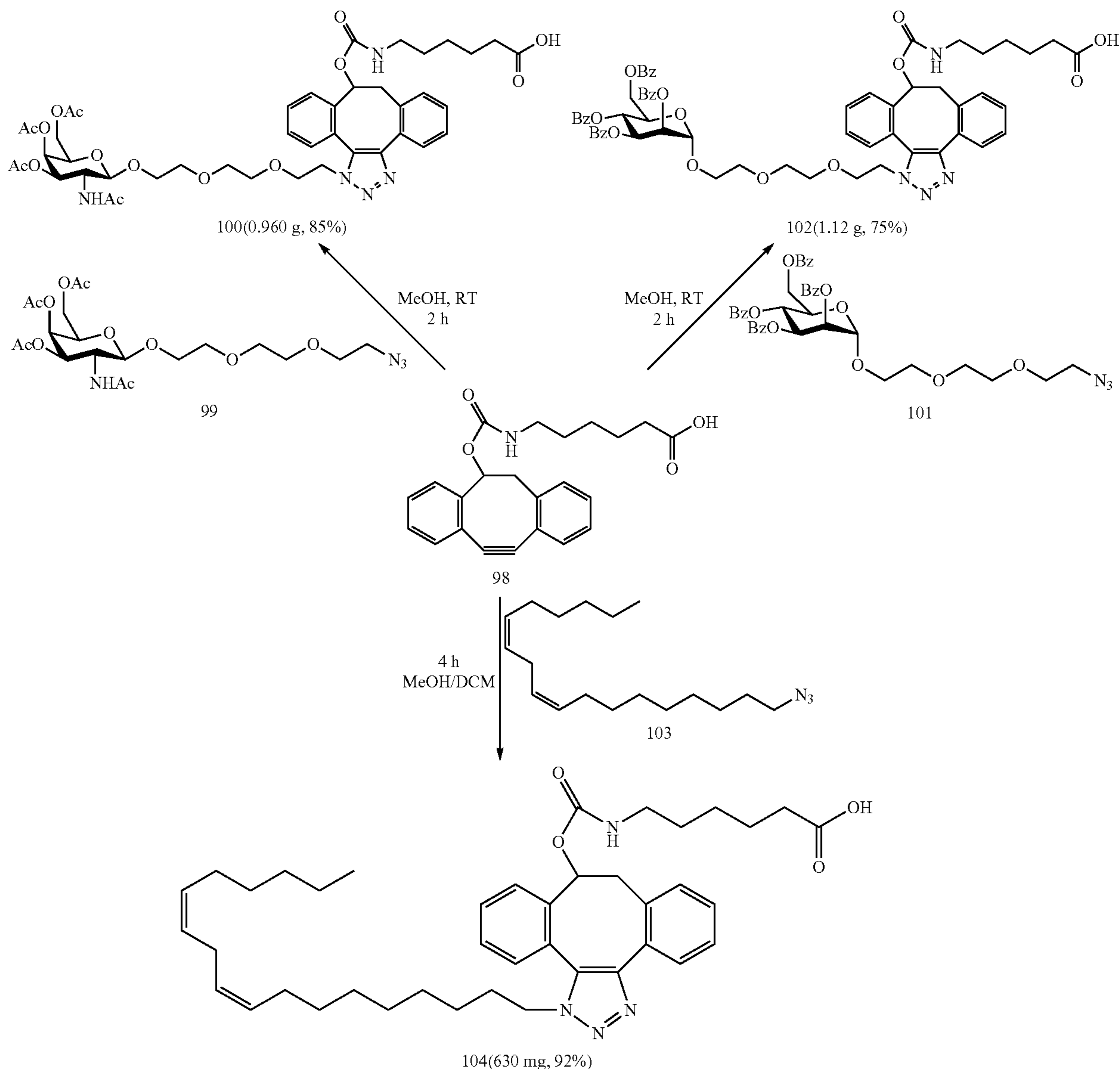
Scheme 2
