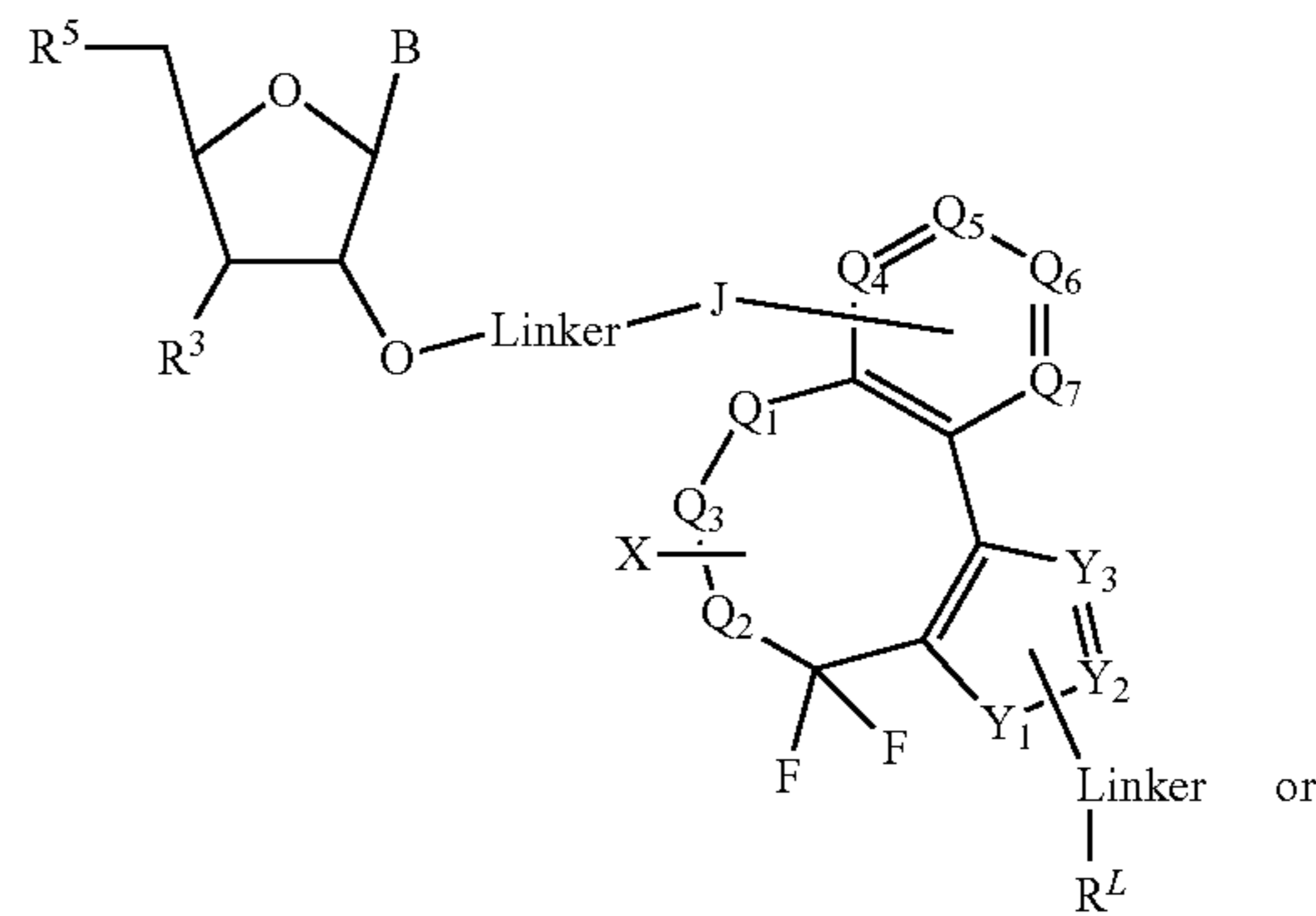
Formula (Vb)
