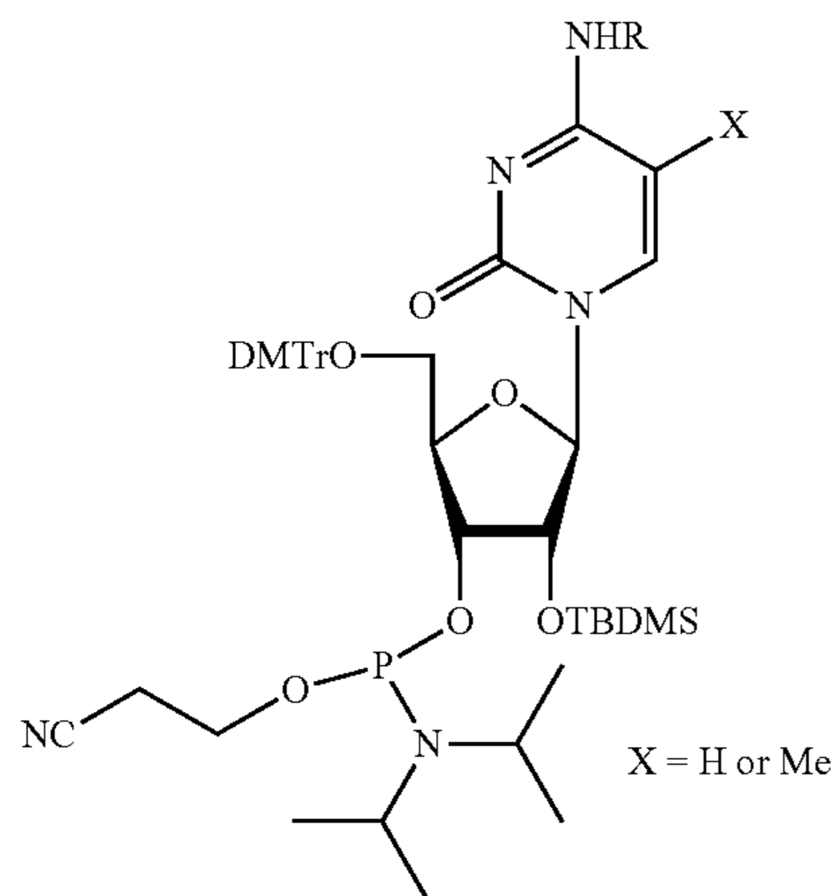
Scheme 16
