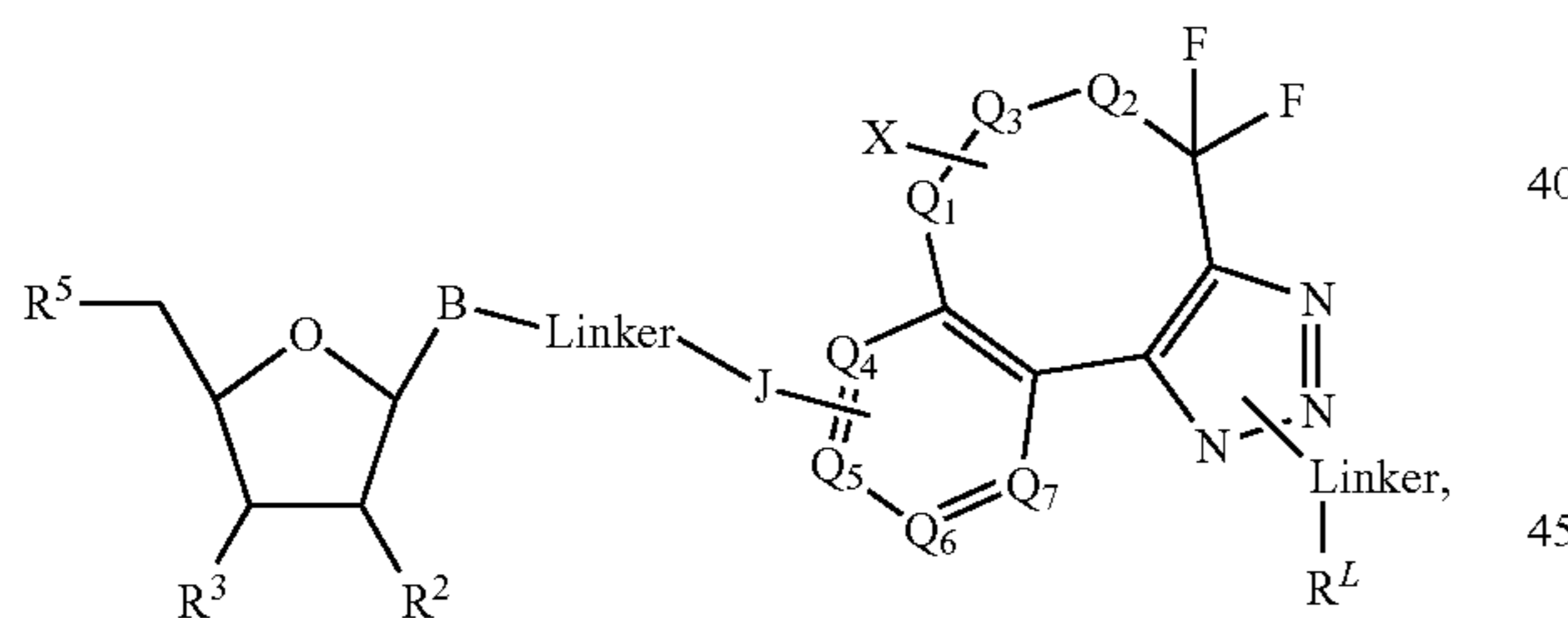
Formula (XVb)
