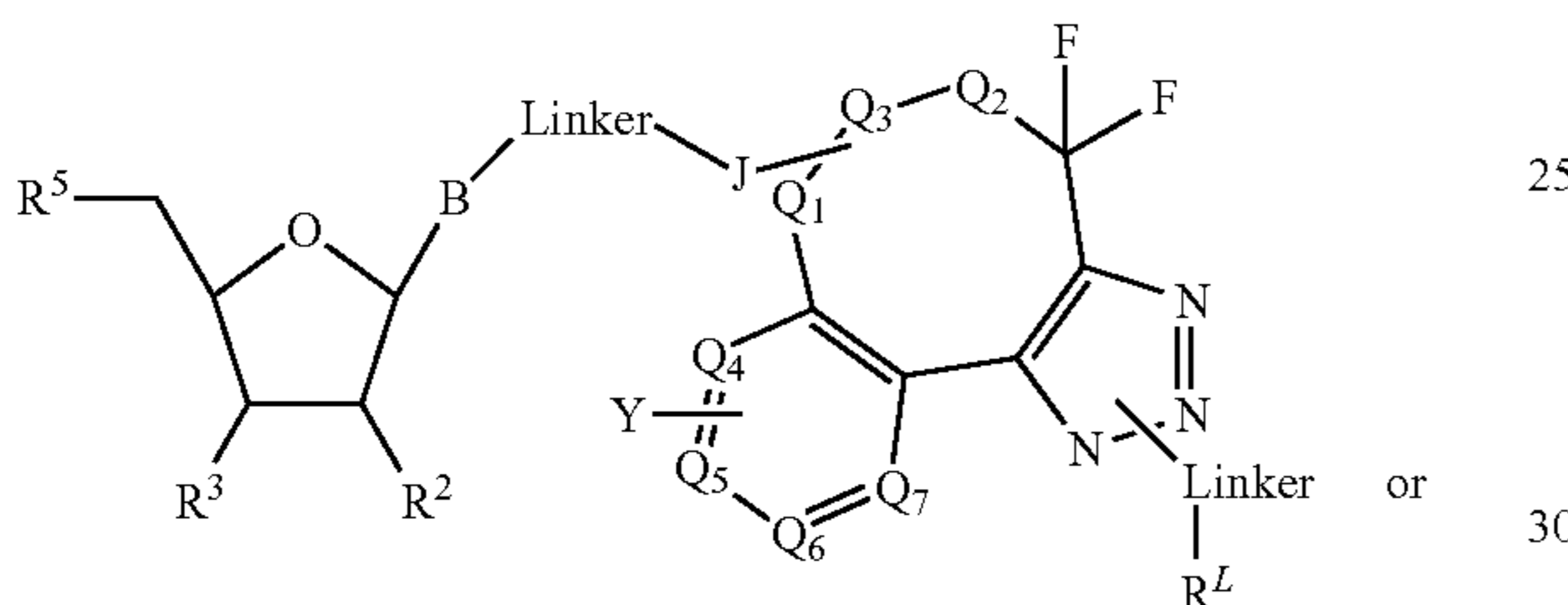
Formula (XVIa)
