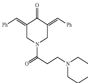
3,5-Di((E)-benzylidene)-1-(3-(piperidin-1-yl)propanoyl)piperidin-4-one (JC003)
