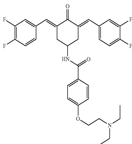
N-(3,5-Bis((E)-3,4-difluorobenzylidene)-4-oxocyclohexyl)-4-(2-(diethylamino)ethoxy)benzamide (JC099)
