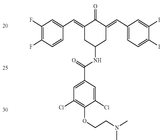
N-(3,5-Bis(E)-3,4-difluorobenzylidene)-4-oxocyclohexyl-4-(2-(dimethylamino)ethoxy)-3,5-dichloro-4-(2-(dimethylamino)ethoxy)benzamide (JC135)
