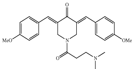
1-(3-(Dimethylamino)propanoyl)-3,5-bis((E)-4-methoxybenzylidene)piperidin-4-one (JC013)
