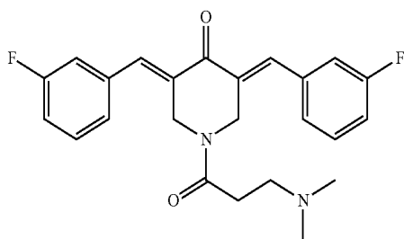
1-(3-(Dimethylamino)propanoyl)-3,5-bis((E)-3-fluorobenzylidene)piperidin-4-one (JC024)
