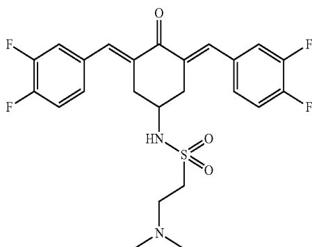
N-(3,5-Bis((E)-3,4-difluorobenzylidene)-4-oxocyclohexyl)-2-(dimethylamino)ethane-1-sulfonamide (JC088)
