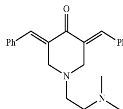
3,5-Di((E)-benzylidene)-1-(2-(dimethylamino)ethyl)piperidin-4-one (JC007)
