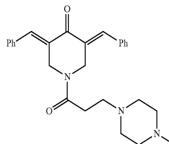
3,5-Di((E)-benzylidene)-1-(3-(4-methylpiperazin-1-yl)propanoyl)piperidin-4-one (JC006)
