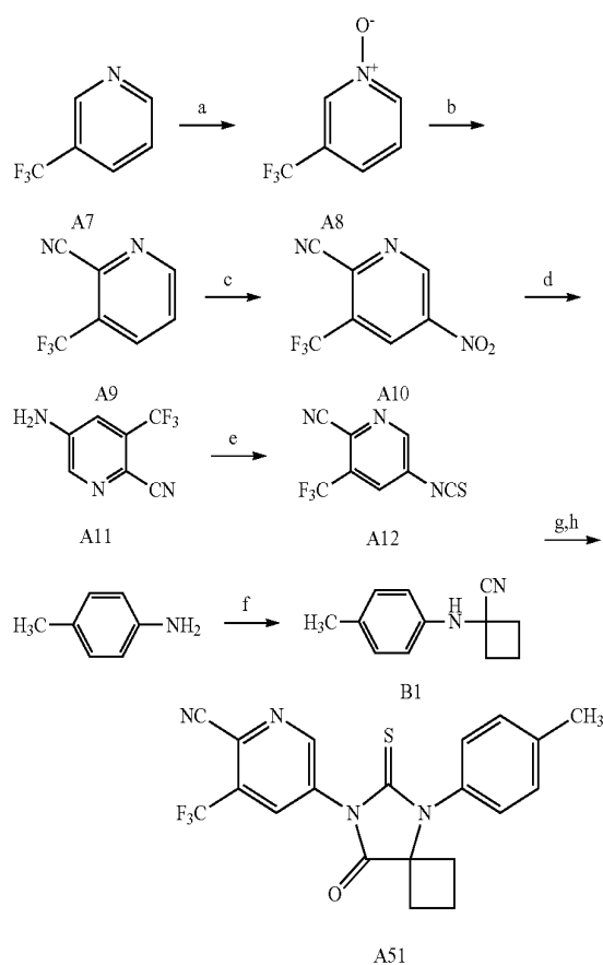
Scheme 2: Synthesis of A51
