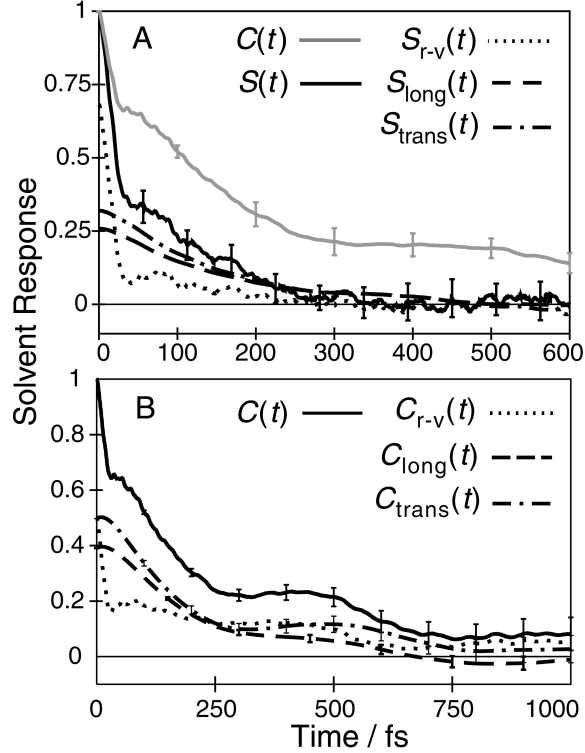
FIG. 1: A. Comparison between the total nonequilibrium, S(t) , and equilibrium, C(t) , solvent response functions, Eqs. 6 and 7, showing the breakdown of LR for the e_{hyd}^- . Integrated projections of the nonequilibrium solvent response onto various (classical) water motions, Eq. 8, are also shown: S_{trans} is the contribution of all COM translations, S_{long} is the projection onto the longitudinal component of the COM translations (see text), and S_{r-v} is the sum of the projections onto the vibrational and rotational motions. The normalization for all of the nonequilibrium curves is \overline{\Delta E}(0) - \overline{\Delta E}(\infty) = 1.47 eV. B. The total equilibrium solvent response function, Eq. 7, and integrated projections of it onto different classical motions, Eq. 9; the subscripts used for each projection are the same as in panel A, except C_{r-v} , which also includes cross-correlations. The error bars shown are \pm 2 standard deviations [16]. The slight difference between the C(t) curves in panels A and B results from a filter ( \exp(-(t/1500\text{fs})^4) ) applied before integrating to obtain the curves in panel B [16].
