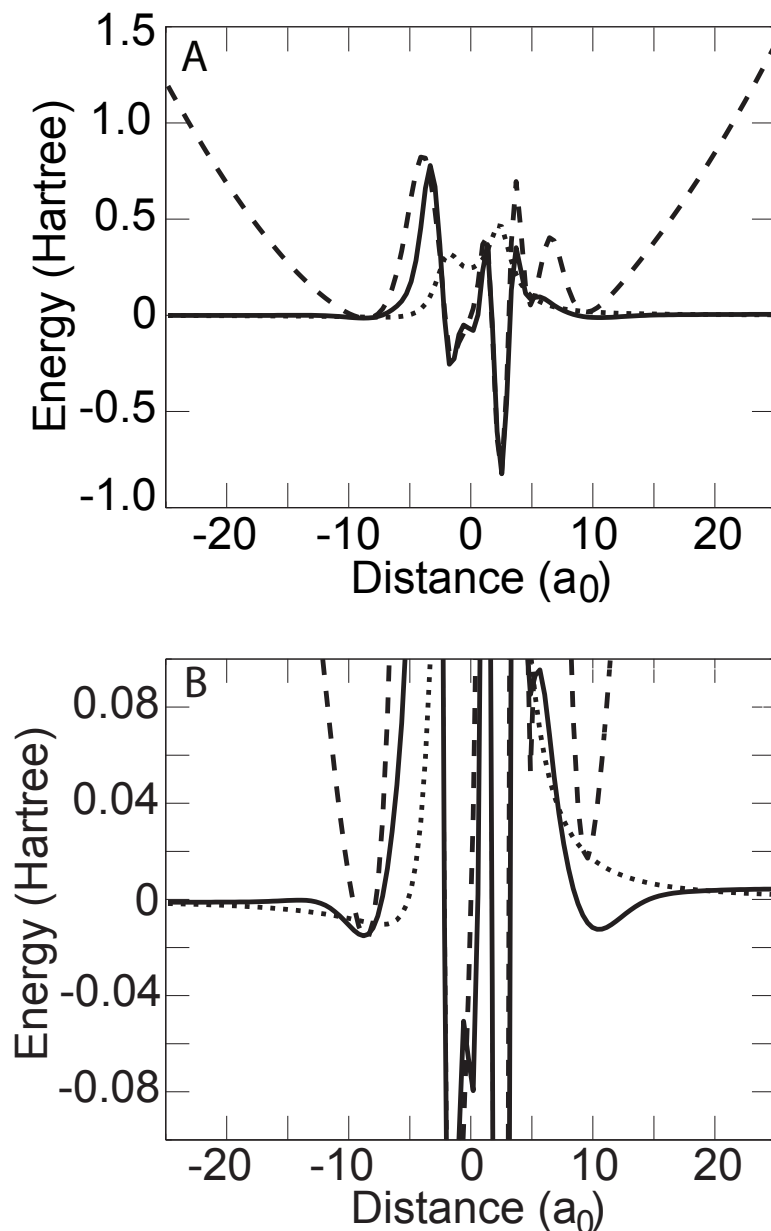
FIG. 2: Correcting the Divergence of THF- e^- Effective Potential at Large Distances Due to the Choice of a Gaussian Basis Set. Panel A shows 1D cuts of the effective potential along the principal symmetry axis of THF calculated using different basis sets: The dashed curve is the effective potential generated with the atom-centered 6-31++G basis set, and the solid curve is the effective potential calculated with a 6-31++G(AUG) basis, which includes off-molecule diffuse basis functions as described in the text. The exact asymptotic long-range potential, \mu/r^3 , is shown as the dotted curve. Use of a non-augmented basis set produces an effective potential whose asymptotic behavior is entirely unphysical (see text). Panel B shows the same data as Panel A but on an expanded scale to facilitate comparison between the different potentials.
