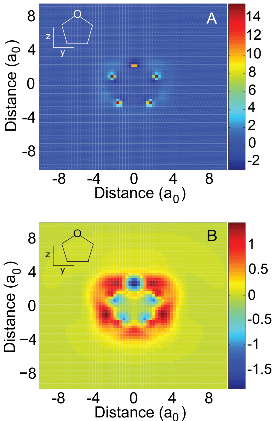
FIG. 3: 2-D Cuts of the Exact Effective e-THF Potential Parallel to the Molecular Plane. The magnitude of the potential in each panel, given by the color scale, is in Hartrees and the spatial axes have units of Bohr radii. The schematic THF molecule drawn in the top left corner of each panel illustrates the perspective of the cut as well as the cartesian axis labels used for the fit described in Table I. The cut in Panel A is 0.16 a_0 above the molecular plane; the cut in Panel B is 0.48 a_0 above the molecular plane. Note that the color scale is not the same in the two panels, and that the magnitude of the potential decays quickly with increasing distance from the molecular plane.
