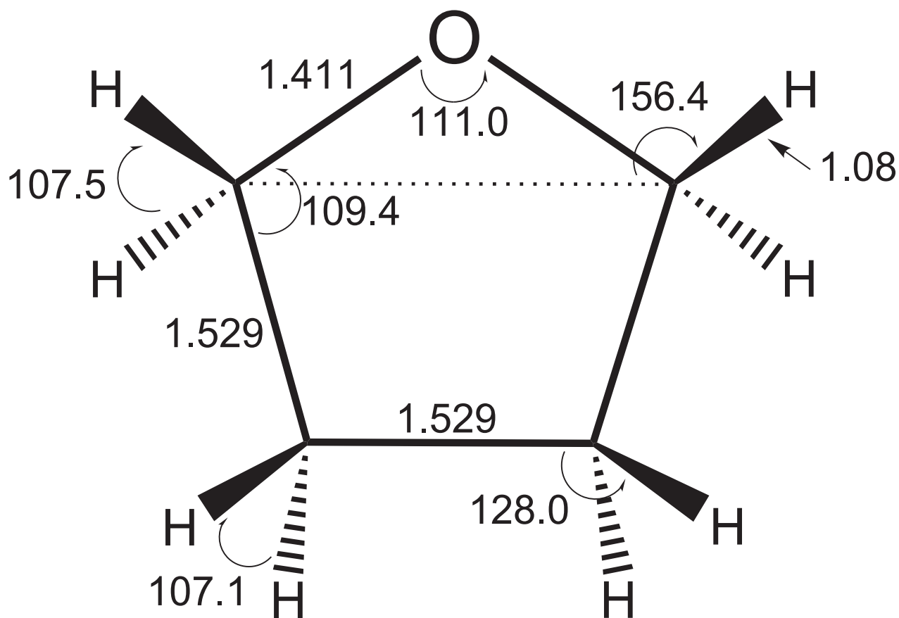
FIG. 1: Hydrogen-optimized Planar THF Structure used in this Work. The bond distances are given in Angstroms ( \text{\AA} ) and angles are in degrees. When projected onto the molecular plan, the alpha hydrogens make a 156.4^\circ angle with respect to the dotted line connecting the alpha carbons and the beta hydrogens form a 128.0^\circ angle with respect to the analogous line connecting the beta carbons.
