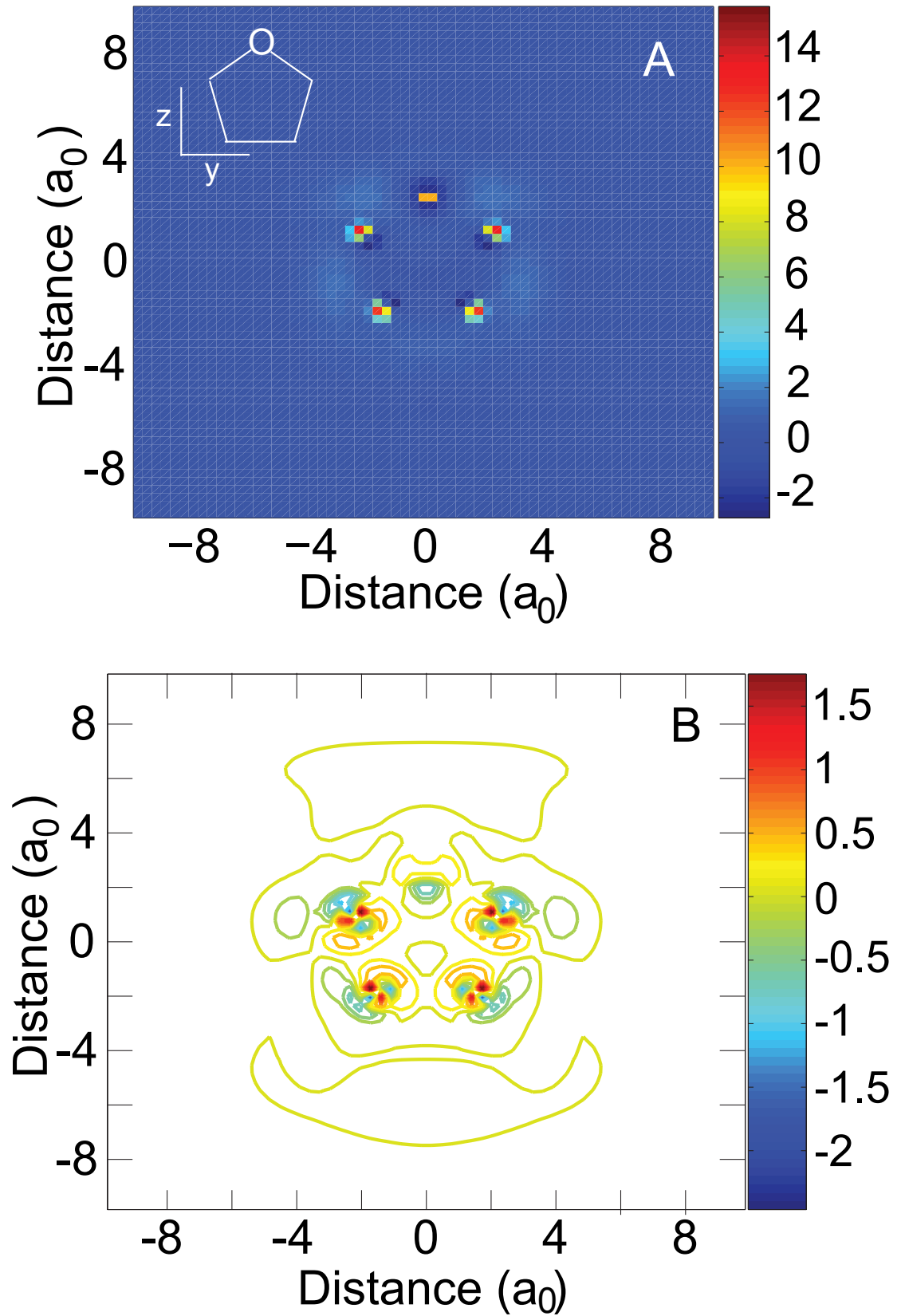
FIG. 5: Fit to the Exact e^- -THF Effective Potential. Panel A shows a 2-D cut of the 55-parameter fit (see Table I and text) parallel to the THF molecular plane and 0.16 a_0 above it; this is the same cut for which the exact effective potential is shown in Figure 3A. Panel B shows the residuals of the fit; i.e. the difference between Figs. 5A and 3A.
