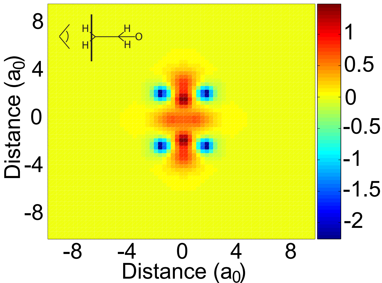
FIG. 4: 2-D Cut of the Exact Effective e-THF Potential Perpendicular to the Molecular Plane. As with Fig. 3, the color scale gives the potential energy in Hartrees and the distance units are in Bohr radii. The viewing perspective of this cut is indicated in the top left corner, where the vertical bar near the \beta -hydrogens represents the plane in which the potential is shown. The strong effect of the hydrogen atoms is clearly visible as the four attractive centers above and below the THF plane.
