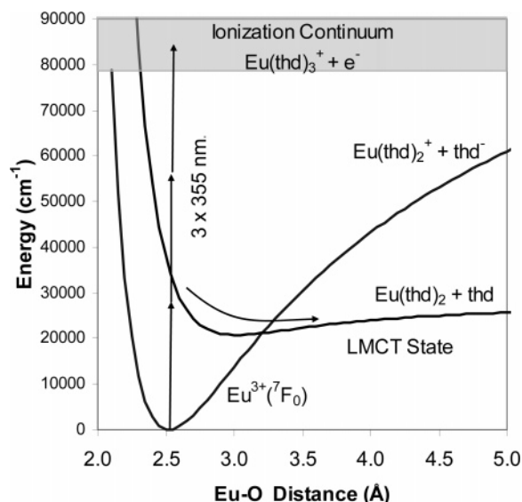
Figure 1. Potential energy diagram for \text{Eu}(\text{thd})_3 , showing multiphoton ionization of the intact molecule in competition with dissociation through the LMCT state into the neutral fragments \text{Eu}(\text{thd})_2 and \text{thd} .
