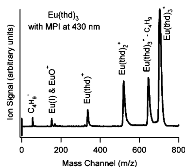
Figure 2. Multiphoton fragmentation and ionization of \text{Eu}(\text{thd})_3 at 430 nm and low fluence ( 10^8 \text{ W/cm}^2 ) showing strong signals for the parent ion and for species resulting from loss of entire ligands from the complex. The parent ion also exhibits a satellite feature representing loss of a tert -butyl group from an attached ligand.
