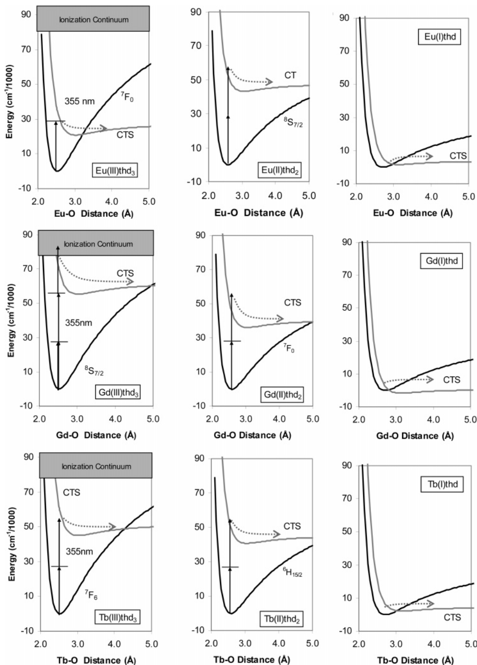
Figure 5. Single-configurational coordinate (SCC) potential energy diagrams for \text{Ln}(\text{thd})_n showing the ground electronic state that correlates with the ionic species \text{Ln}(\text{thd})_{n-1}^+ + \text{thd}^- and the excited LMCT state that correlates with the neutral fragments \text{Ln}(\text{thd})_{n-1} + \text{thd} . Vertical arrows represent absorbance of 355-nm photons. Vertical optical transitions to the LMCT are predicted to result in formation of the complex on the repulsive wall and above the dissociation limit of the LMCT, resulting in dissociation of the intact (neutral) ligand fragment. This dissociation is illustrated by the curved dashed-line arrows. The first panel in each row illustrates dissociation of the parent \text{Ln}(\text{thd})_3 into products \text{Ln}(\text{thd})_2 + \text{thd} . The second panel illustrates the dissociation of that \text{Ln}(\text{thd})_2 product, yielding \text{Ln}(\text{thd}) + \text{thd} . The third panel then illustrates the dissociation of the monoligated \text{Ln}(\text{thd}) , yielding the bare metal atom, \text{Ln}(0) , and the neutral thd ligand radical. The greatest difference between the three metals in the energies of the LMCT occurs for the first dissociation step (first panel).
