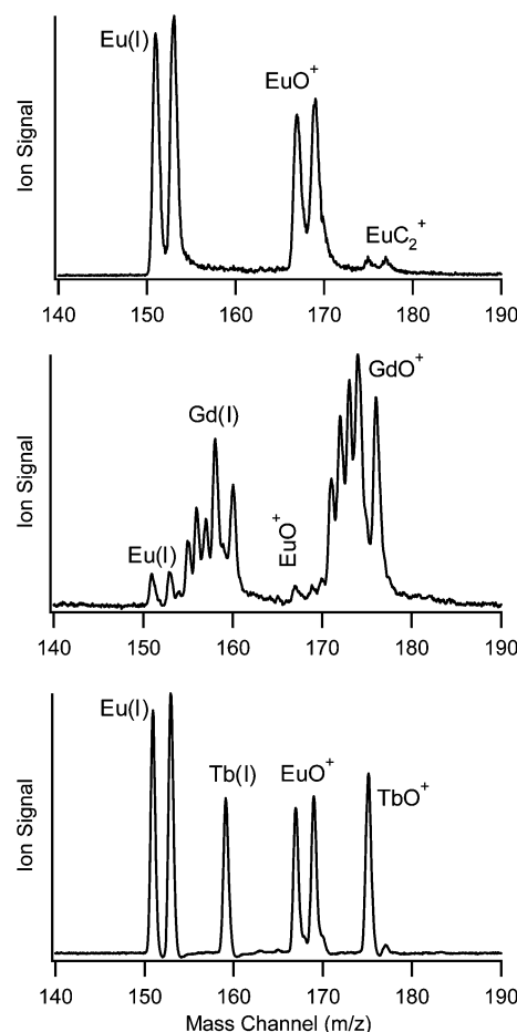
Figure 4. Photoionization of \text{Ln}(\text{thd})_3 at 355 nm and low fluence ( \sim 10^8 W/cm 2 ). The \text{Ln}(\text{II}) signal at this fluence is small. At higher fluence, both \text{Ln}(\text{I}) and \text{LnO}^+ are converted to \text{Ln}(\text{II}) . The differences in the \text{Ln}(\text{I}) -to- \text{LnO}^+ ion-signal ratio reflect the relative accessibility of the LMCT state for the three metals.
