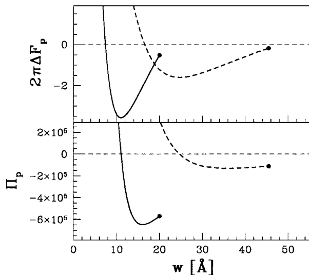
Figure 13. Polyelectrolyte contribution to (a) the interaction free energy, 2\pi\Delta F_p (eq 31) and (b) the intersurface force, \Pi_p (eq 32), in the low-salt regime as function of the intersurface separation w . Same physical values, notations, and units as in Figure 6. The numerical prefactors of the intermediate profile h_3(z, \eta) with \eta = 3/2 were used in the calculation of the interaction free energy and forces, and the numerical prefactors of the parabolic profile were used in the calculation of the single surface free energies. Solid line p = 1 ; dashed line p = 0.2 .
