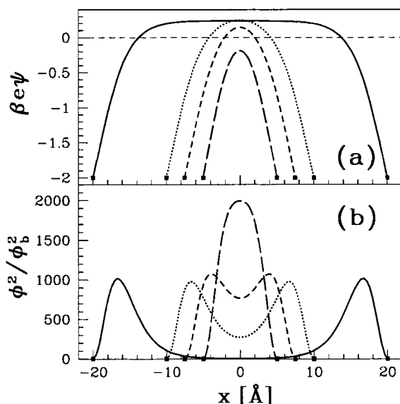
Figure 3. Profiles of (a) the reduced electrostatic potential y = \beta\psi and (b) the reduced monomer concentration \phi^2/\phi_b^2 as functions of the position x between the two surfaces. The profiles were obtained by solving numerically the differential equations (eqs 5 and 6) for several intersurface distances. For comparison, the different profiles are plotted on the same axis so that all midplanes ( x = 0 ) coincide. The surfaces are placed at different distances from the midplane, and their positions are indicated by the filled squares. In the numerical examples in Figures 3–11, we assume the following physical parameters. The polymer concentration is \phi_b^2 = 10^{-6} \text{ Å}^{-3} with an effective monomer length a = 5 \text{ Å} and excluded volume parameter \nu = 50 \text{ Å}^3 . It is immersed in an aqueous solution ( \epsilon = 80 ) at room temperature ( T = 300 \text{ K} ) and the surfaces are kept at a constant potential y_s = \beta\psi_s = -2 . In addition, in the current figure, the polymer charge fraction p = 1 and the salt concentration c_b = 1 \text{ mM} . The different curves correspond to separations of w = 40 \text{ Å} (solid curve); w = 20 \text{ Å} (dots); w = 15 \text{ Å} (short dashes), and w = 10 \text{ Å} (long dashes).
