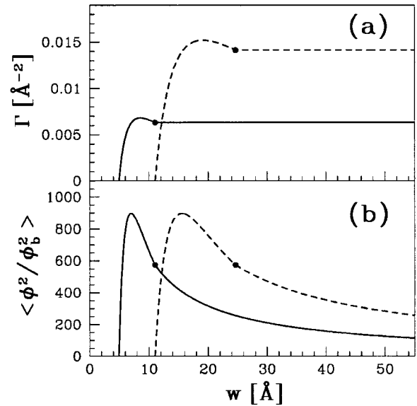
Figure 12. Adsorption of polyelectrolytes in the low-salt regime as calculated from eqs 29 and 30. (a) Total amount of monomers adsorbed between the surfaces per unit area \Gamma , and (b) the average reduced monomer concentration \langle \phi^2 / \phi_b^2 \rangle as function of the intersurface distance w . The physical values and notations are the same as in Figure 4. The numerical prefactors of the intermediate profile h_3(z, \eta) with \eta = 3/2 were used in the calculation. The vertical lines denote the distance where w = 2D_1 .
