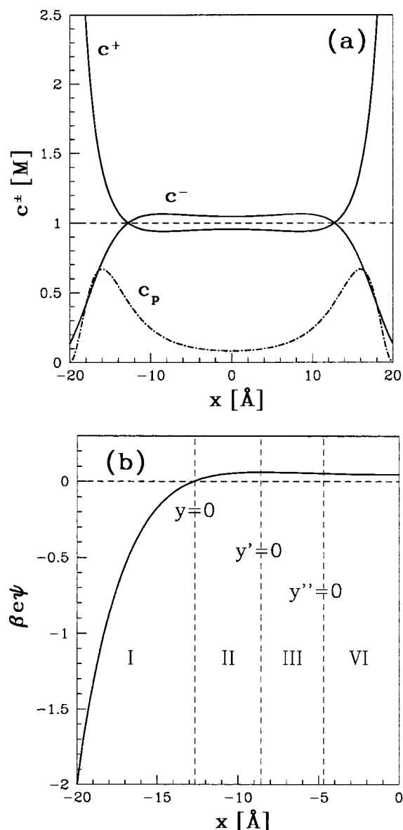
Figure 8. (a) Profiles of the charge concentrations: c^+ , c^- , and c_p = p\phi_b^2 , as functions of the position x between the two surfaces for w = 40 Å. The reduced electrostatic potential \beta e\psi between one of the surfaces and the midplane is plotted in (b). The special points y = 0 , y' = 0 and y'' = 0 are marked.
