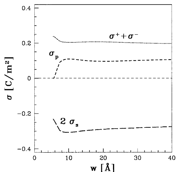
Figure 9. Different contributions to the total charge density per unit area as a function of the intersurface distance w for highly charged polyelectrolytes ( p = 1 ) in the high-salt limit ( c_b = 1 M). The different curves correspond to twice the induced surface charge density 2\sigma_s , the total amount of polymer charge adsorbed between the two surfaces per unit area \sigma_p , and the total amount of charge carried by small ions ( \sigma^+ + \sigma^- ).
