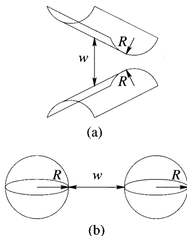
Figure 2. (a) Two half cylinders with a 90° tilt between the axes, as used in the surface force apparatus to measure intersurface forces. The radii R of the cylinders are of the order of 1–2 cm, while w ranges down to a few angstroms. (b) Two spheres of radii R at a distance w . Typically, colloidal suspensions contain particles whose radii are of a few micrometers down to hundreds of angstroms, while the stability is determined by the balance of forces at much smaller distances.
