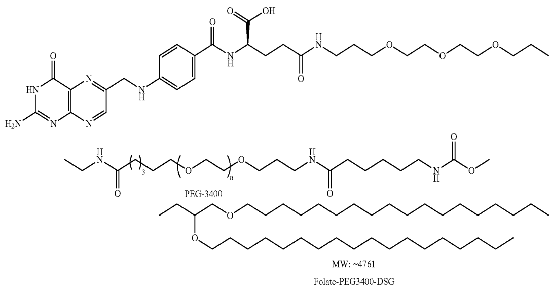
Formula 7
