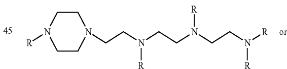
formula (IV)
