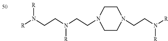
formula (IV)
