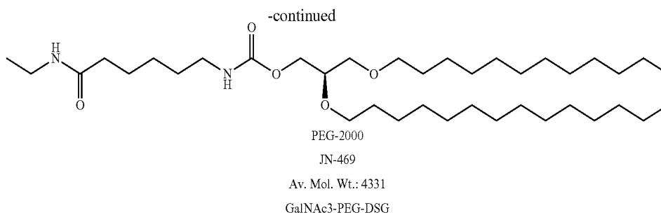
Formula 6
