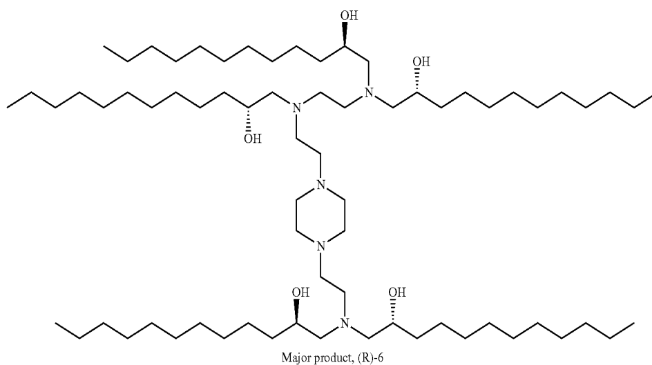
Scheme 7
