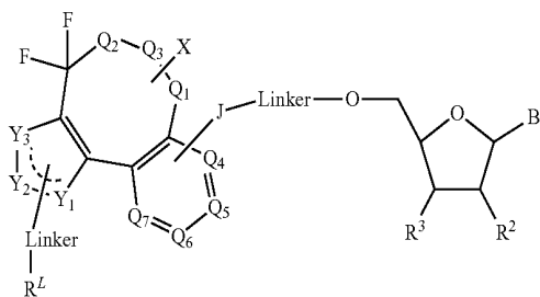
Formula (IXb)
