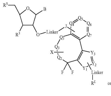
Formula (Vb)
