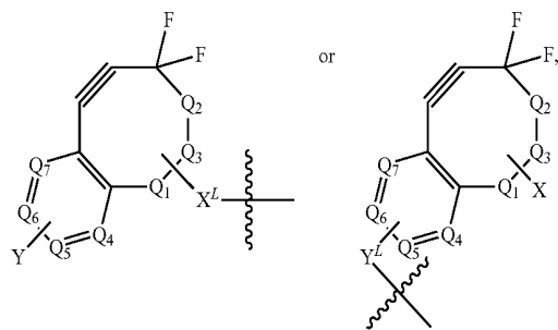
Formula (XI)
