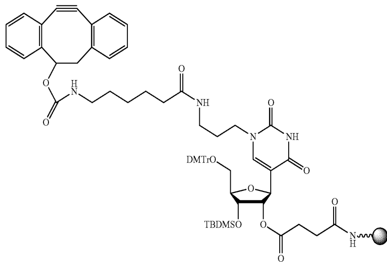
Scheme 20
