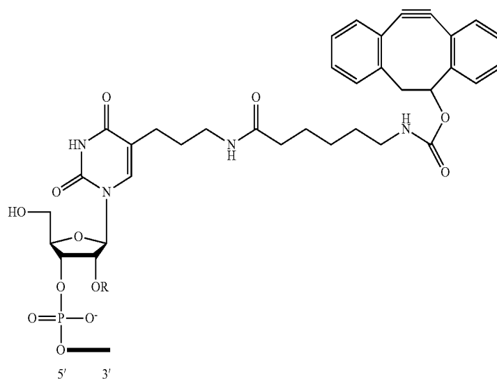
Scheme 18
