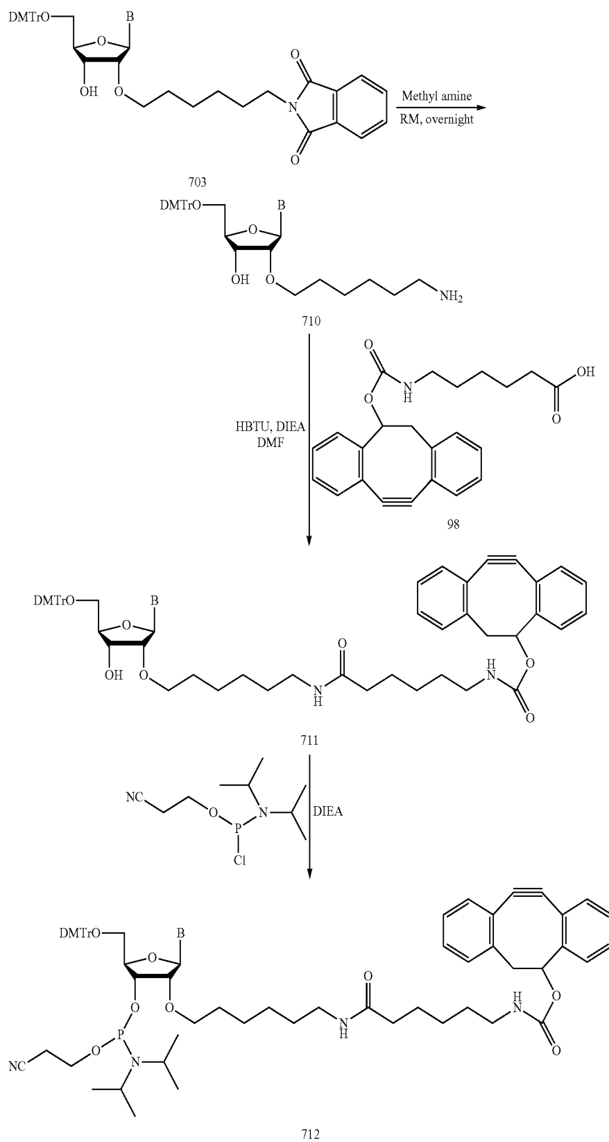
Scheme 14
