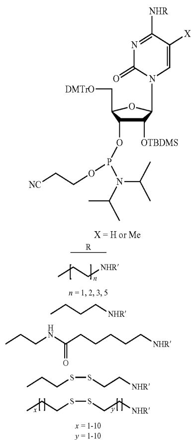
Scheme 16
