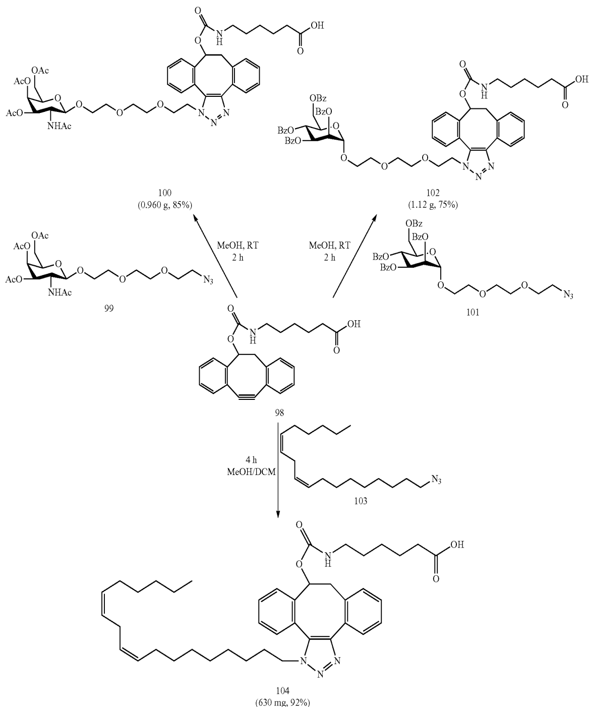
Scheme 2
