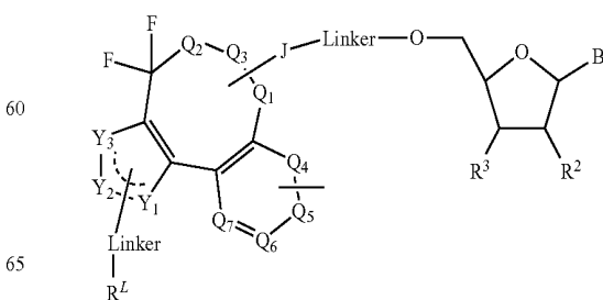
Formula (IXa)
