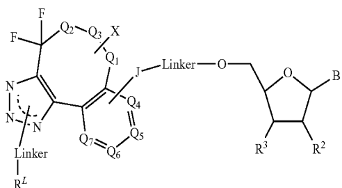
Formula (Xb)
