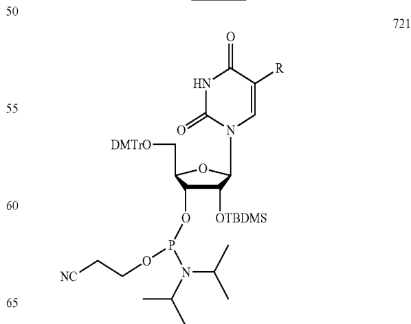
Scheme 17
