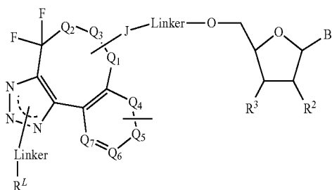
Formula (Xb)
