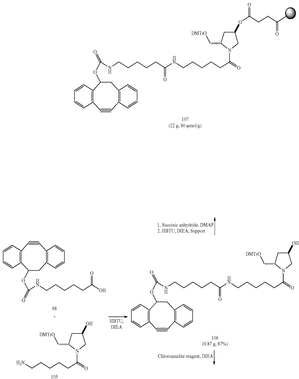
Scheme 3
