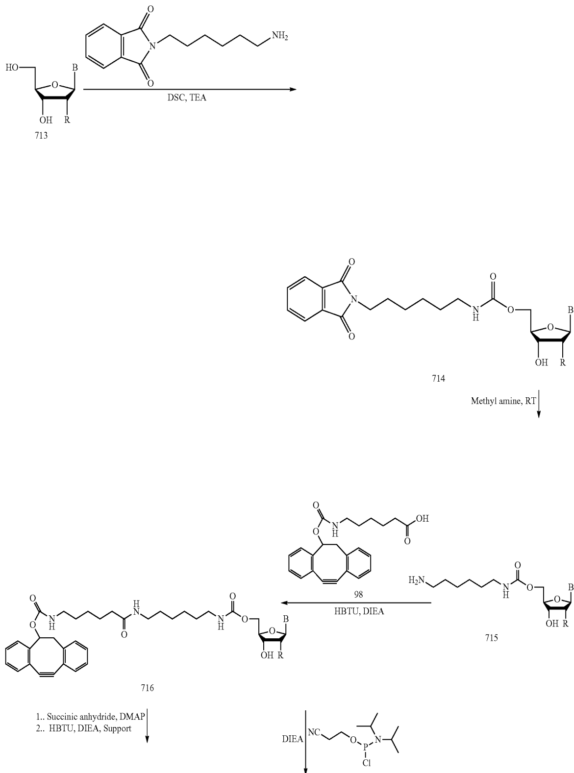
Scheme 15
