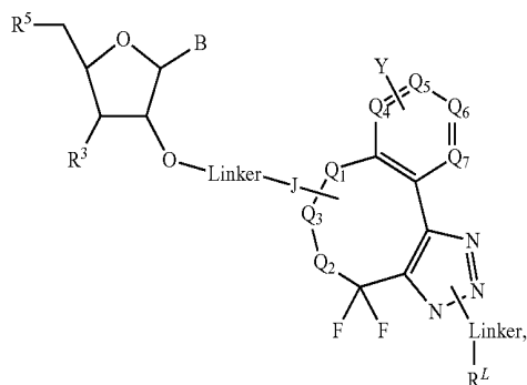
Formula (VIb)
