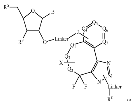
Formula (VIa)
