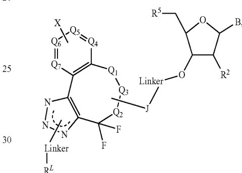
Formula (VII)
