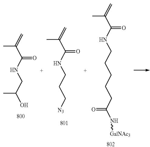
Scheme 21
