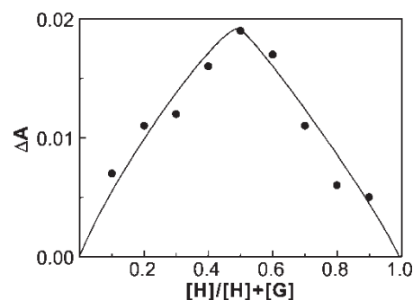
FIGURE 2 A Job plot for the complexation of 2 (H) with bile salt CA (G) in a Tris buffer solution (pH 7.4) at 25°C ( [H] + [G] = 5.0 \times 10^{-4} \text{ M} ).
