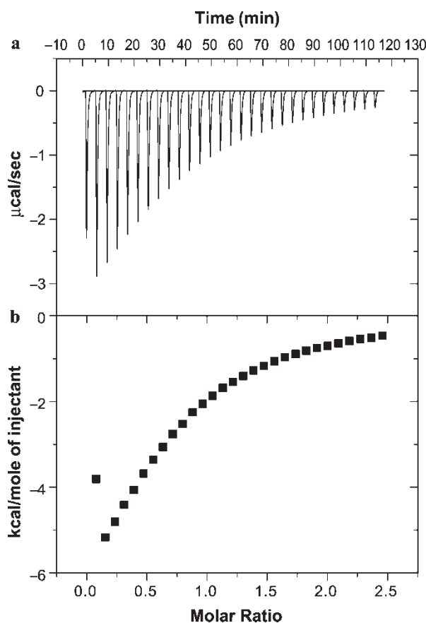
FIGURE 1 Calorimetric titration of dimer 1 with bile salt DCA in Tris buffer (pH 7.4) at 25°C. (a) Raw data for sequential 10 \mu\text{L} injections of cyclodextrin (2.19 mM) into bile salt solution (0.2 mM). (b) Heats of reaction as obtained from the integration of the calorimetric traces.
