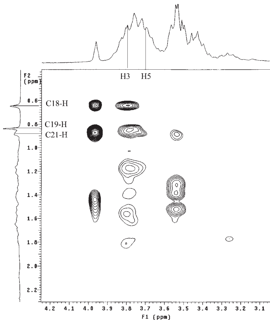
FIGURE 4 Partial 1 H ROESY spectrum (300 MHz) of a mixture of cyclodextrin 1 (1.5 mM) and DCA (1.5 mM) in D 2 O at 298.1 K with a mixing time of 600 ms.
