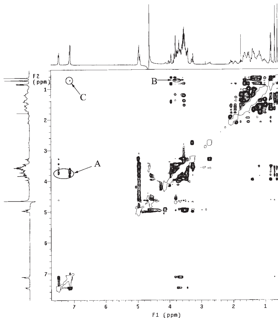
FIGURE 7 1 H ROESY spectrum (300 MHz) of a mixture of cyclodextrin 4 (1.5 mM) and bile salt DCA (1.5 mM) in D 2 O at 298.1 K with a mixing time of 600 ms.
