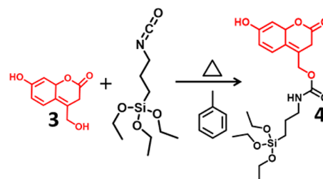
Figure 3. Synthesis of the silane-modified coumarin molecule.
